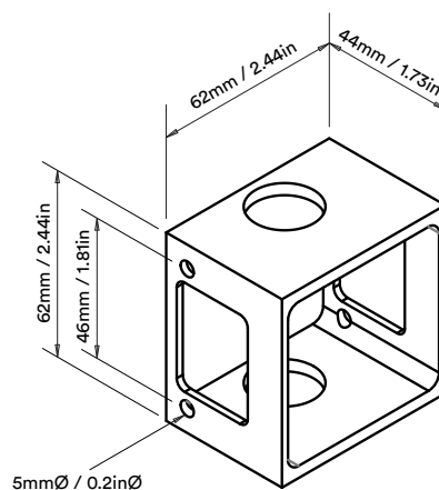
Optional back box for masonry applications only
